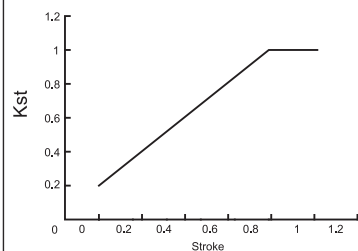
Short stroke factor diagram
